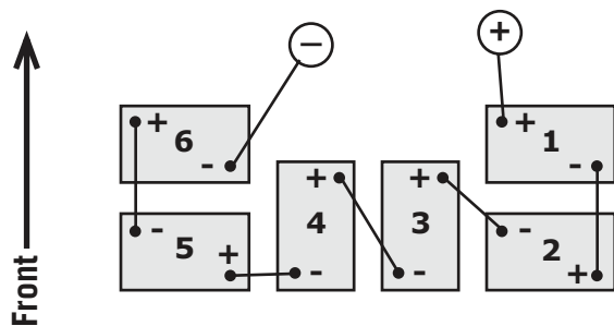
(Fig. F) EZGO TXT Model 36-Volt Battery Pack
